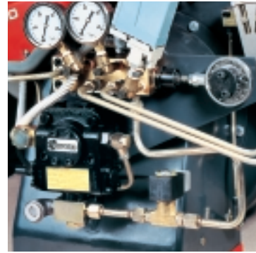
Example of the hydraulic circuit on RL70/M burners
